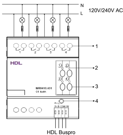
Figure 4. Wiring
