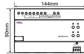
4CH 1.5A MOSFET Dimming Actuator Figure 5. Dimensions - Front View
