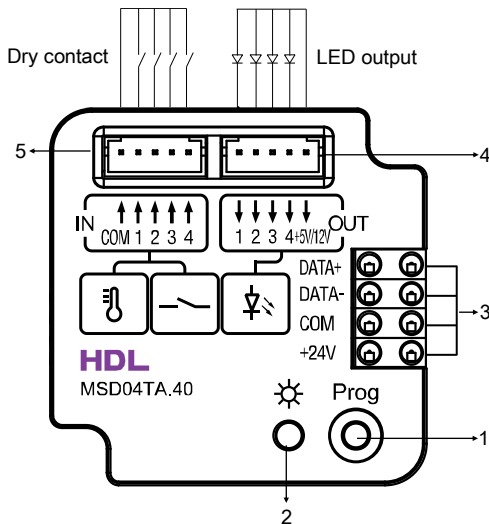
Figure 4. Wiring
