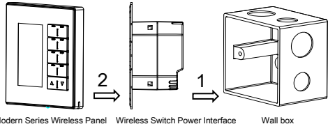
Figure 9. Installation
