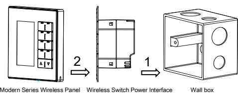
Figure 9. Installation
