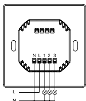
Figure 7. Wiring (1)
