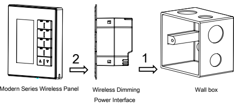
Figure 9. Installation
