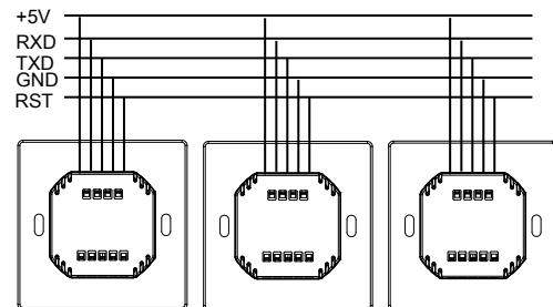
Figure 8. Wiring (2)
