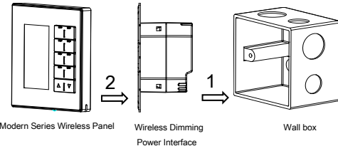
Figure 9. Installation
