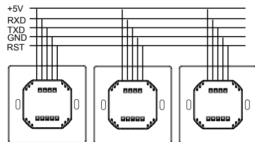
Figure 8. Wiring (2)
