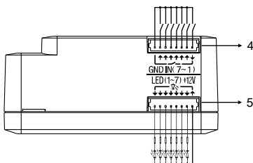
Figure 5. Wiring
