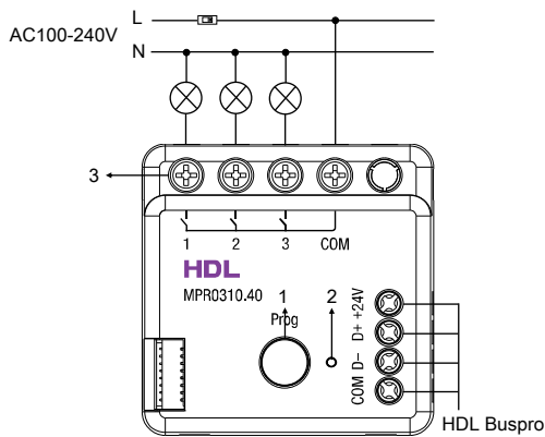
Figure 4. Wiring
