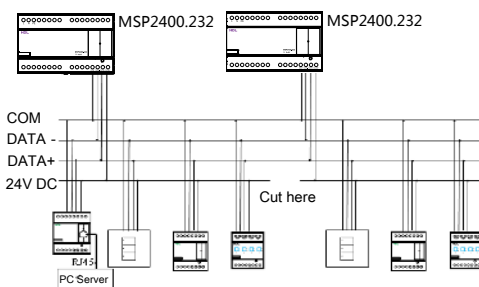
Figure 4. Wiring
