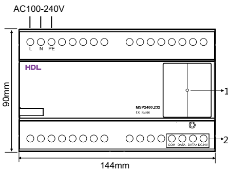
Figure 2. Dimensions - Front View
