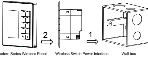
Figure 10. Installation
