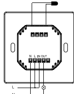
Figure 8. Wiring (1)
