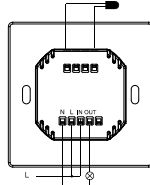
Figure 8. Wiring (1)
