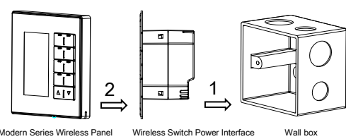
Figure 10. Installation
