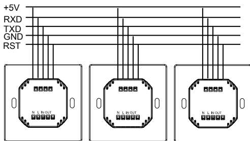
Figure 9. Wiring (2)
