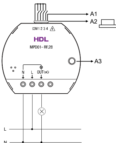
Figure 4. Wiring
