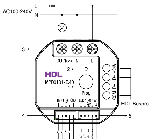
Figure 4. Wiring
