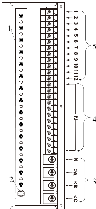
Power input and load wiring terminal
