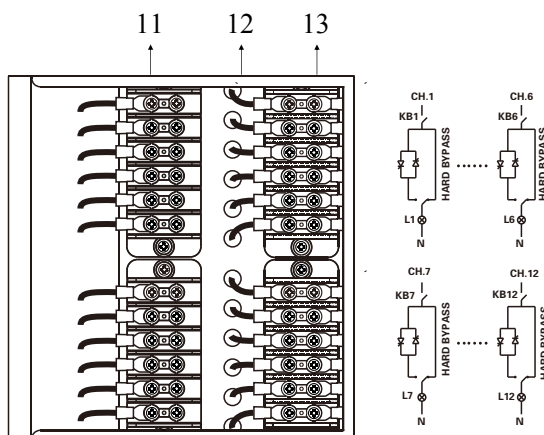
Jumper wiring terminal
