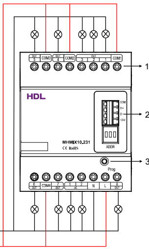
Figure 4. Wiring
